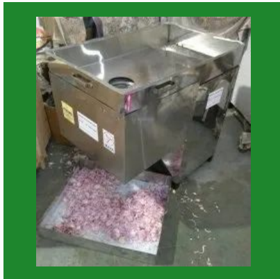
Automatic Onion Slicer Machine
